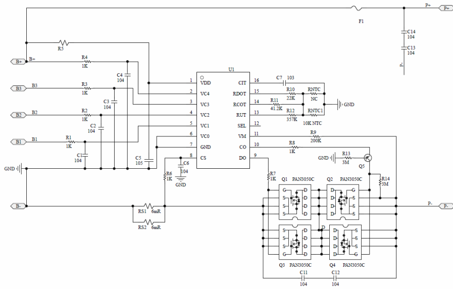
Circuit diagram
