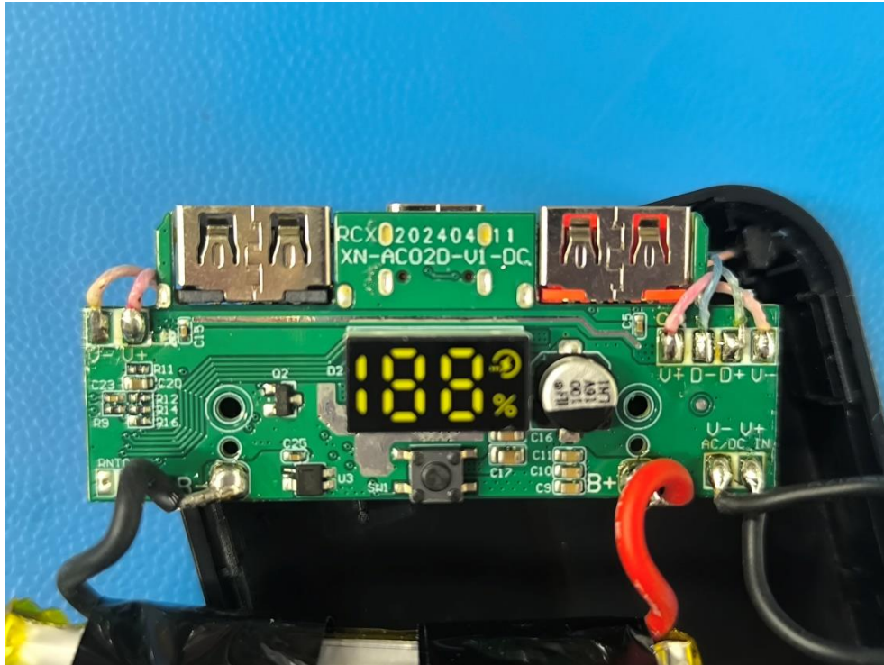
Figure 9_ Internal view for AC-02F
