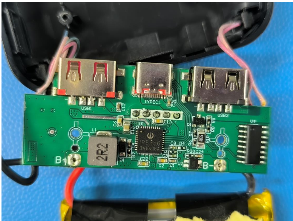
Figure 10_ Internal view for AC-02F
