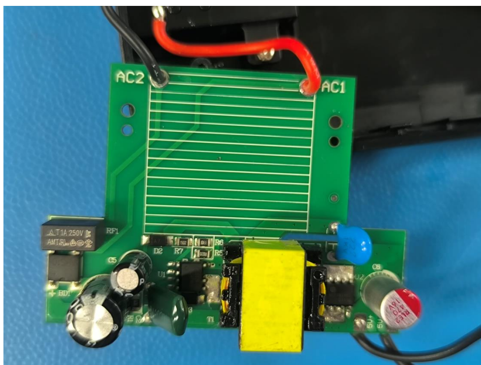
Figure 8_ Internal view for AC-02F
